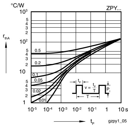
Figure 2. Pulse Thermal Resistance vs. Pulse Duration
