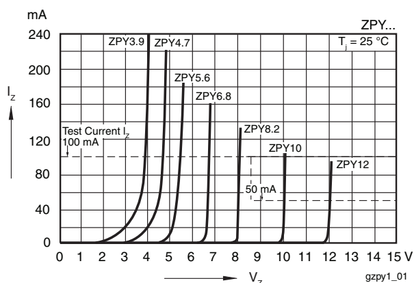
Figure 7. Breakdown Characteristics
