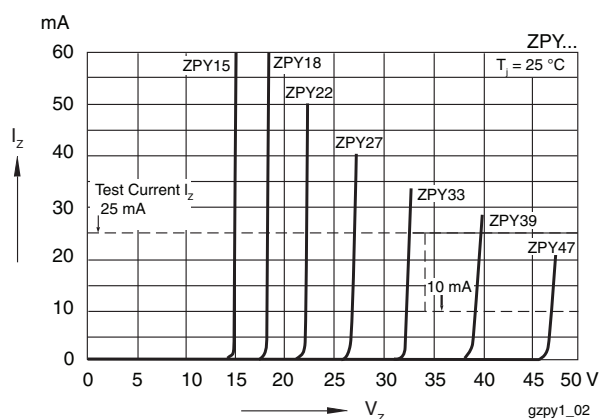
Figure 8. Breakdown Characteristics
