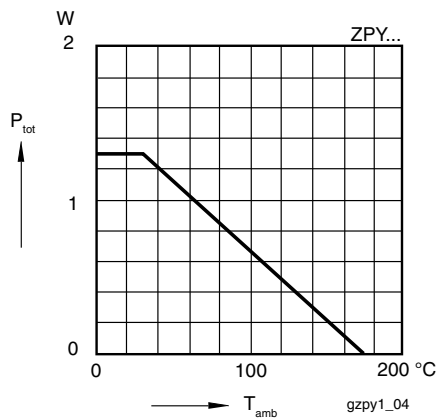
Figure 1. Admissible Power Dissipation vs. Ambient Temperature
