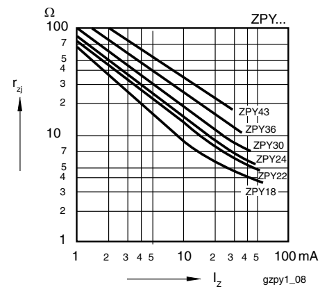
Figure 5. Dynamic Resistance vs. Zener Current
