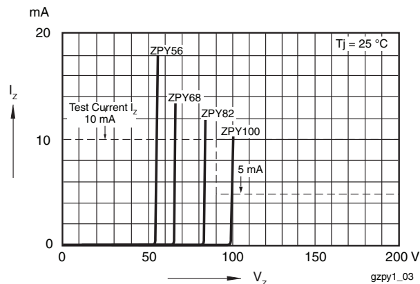
Figure 9. Breakdown Characteristics
