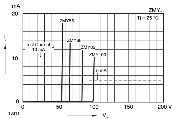
Fig. 8 - Breakdown Characteristics
