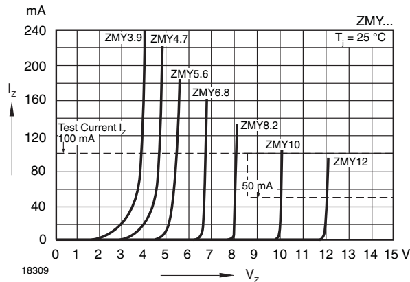
Fig. 6 - Breakdown Characteristics
