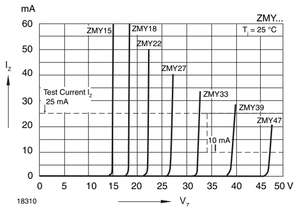
Fig. 7 - Breakdown Characteristics
