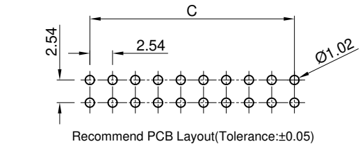
Recommend PCB Layout(Tolerance:±0.05)
