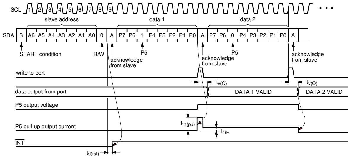
Fig 7. Write mode (output)
