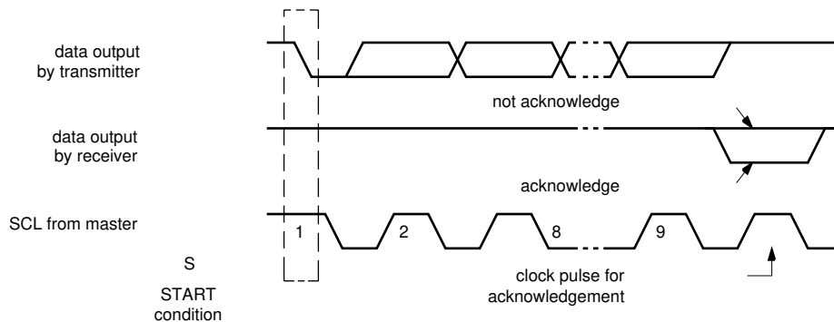
Fig 13. Acknowledgement on the I²C-bus
