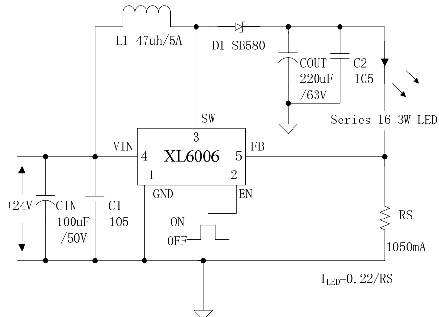
Figure7. XL6006 System Parameters Test Circuit (24V ~ 16 x 3W LED)
