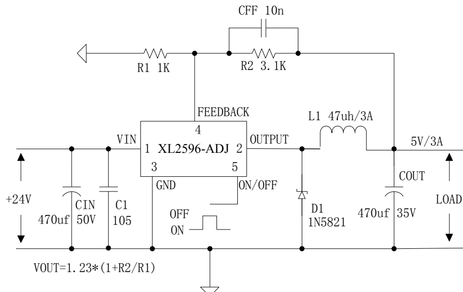
Figure9. XL2596-ADJ System Parameters Test Circuit
