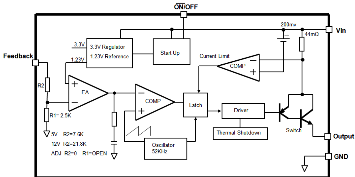
Figure3. Function Block Diagram of XL2576
