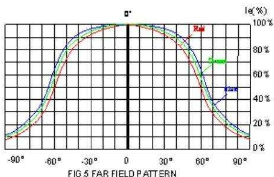
FIG 5 FAR FIELD PATTERN
