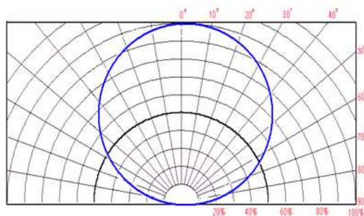
Directive Characteristics ( T_a=25^\circ\text{C} )
