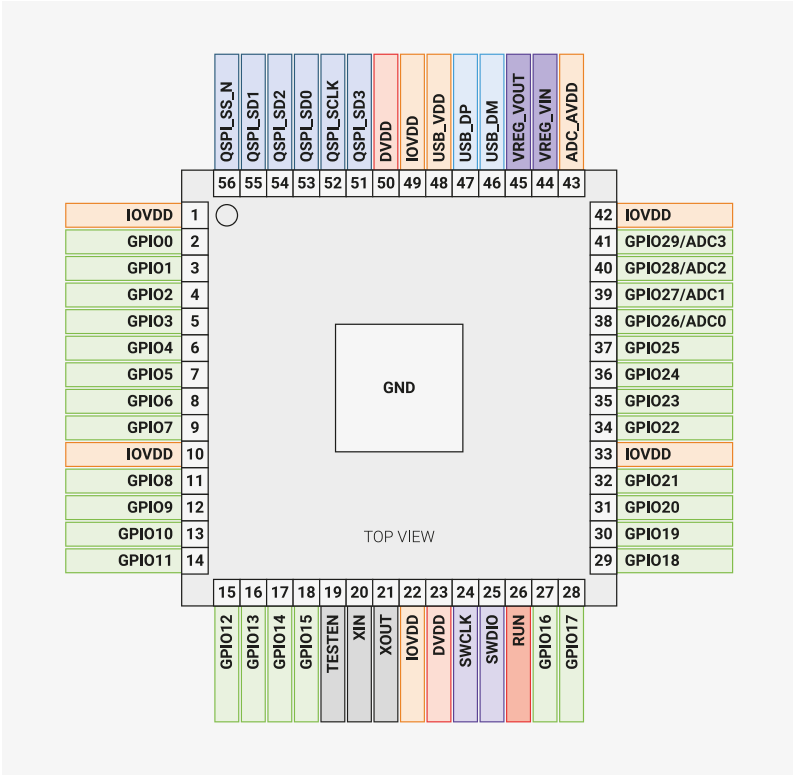
Figure 168. RP2040 QFN-56 package pinout
