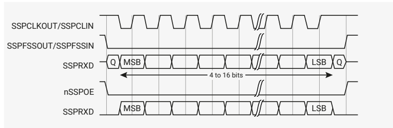
Figure 95. Motorola SPI frame format with SP0=1 and SPH=1 , single and continuous transfers
