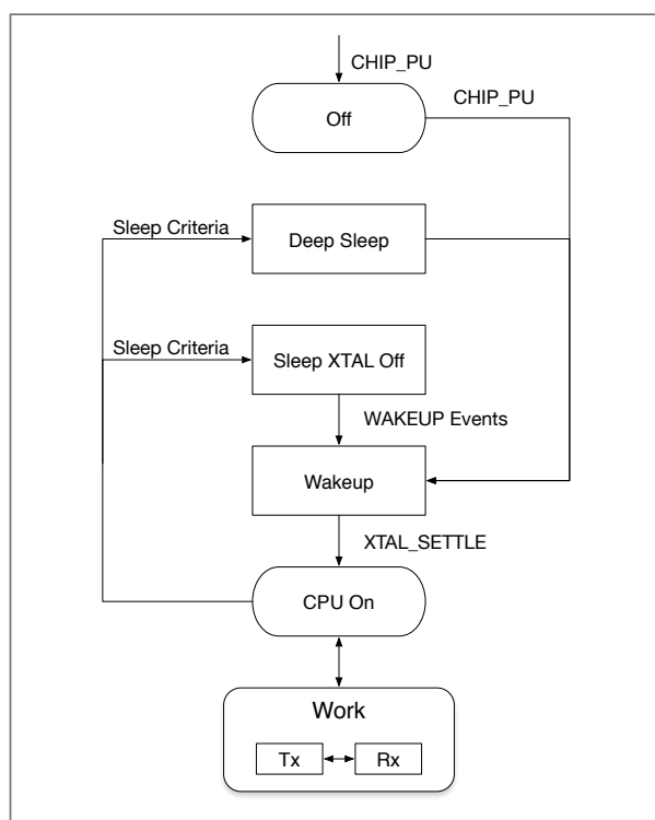
Figure 3-2. Power Management
