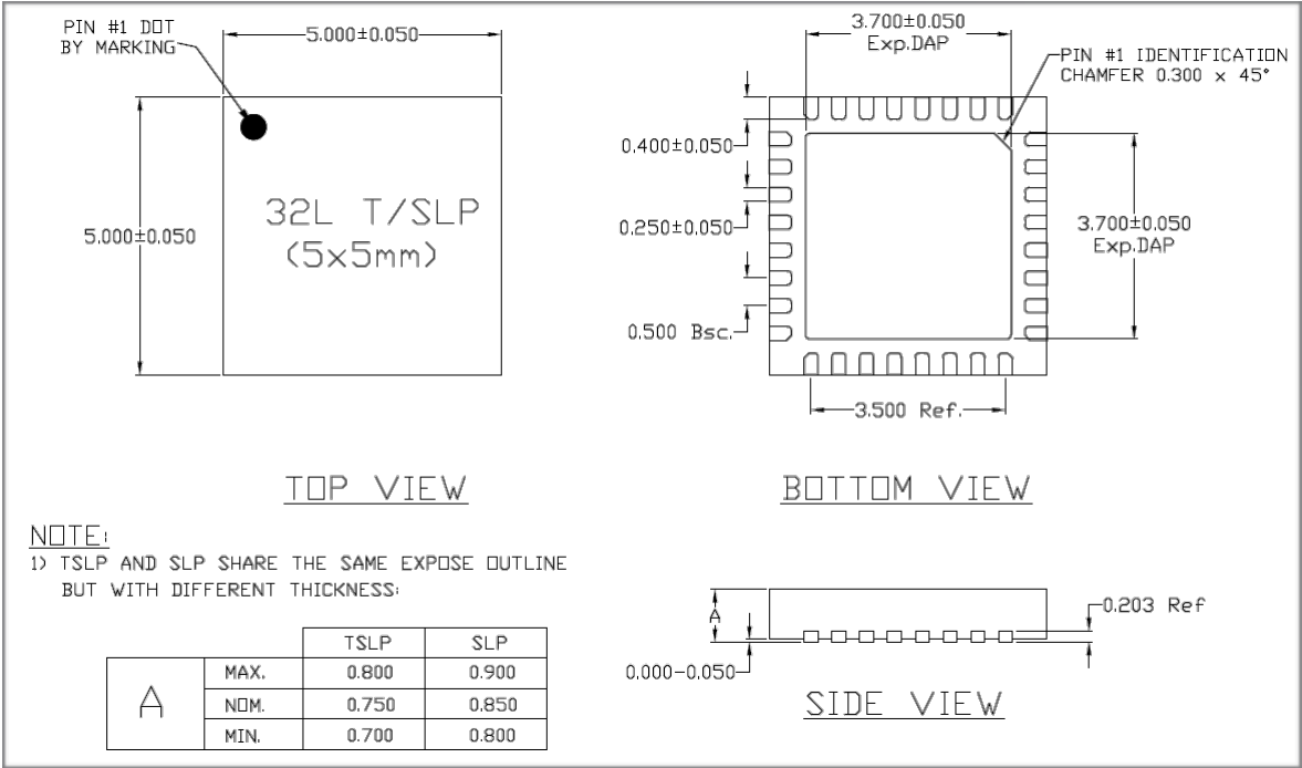
Figure 6-1. ESP8266EX Package
