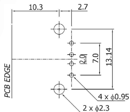
PCB Layot (bottom view)
