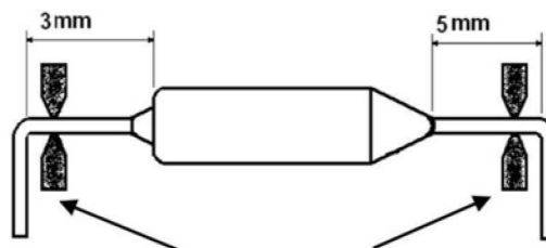
Stationary Fixture
