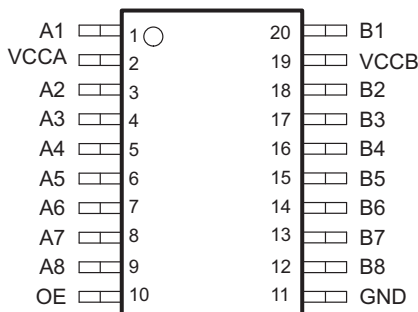
PW Package 20-Pin TSSOP (TOP VIEW)
