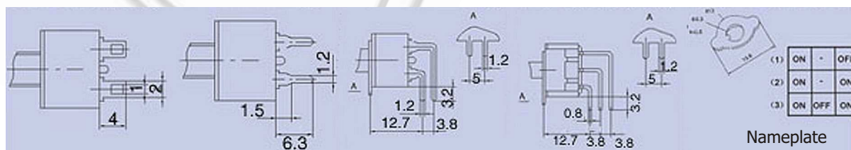
Solder terminal (1) PC terminal (2) PC-H terminal (3) PC-V terminal (4)
