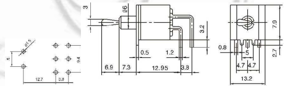
TSM202C3 ON-ON TSM212C3 ON-(ON) TSM203C3 ON-OFF-ON TSM213C3 ON-OFF-(ON) TSM223C3 (ON)-OFF-(ON) DPDT 6P
