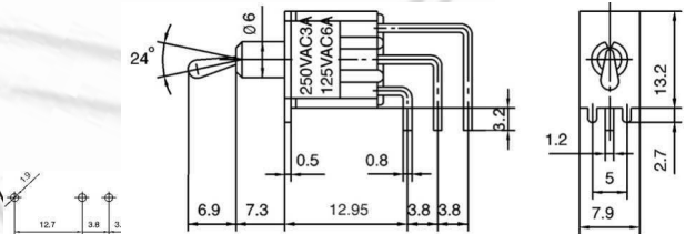
TSM102C4 ON-ON TSM112C4 ON-(ON) TSM103C4 ON-OFF-ON TSM113C4 ON-OFF-(ON) TSM123C4 (ON)-OFF-(ON) SPDT 3P
