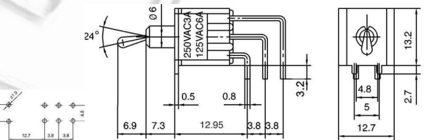
TSM202C4 ON-ON TSM212C4 ON-(ON) TSM203C4 ON-OFF-ON TSM213C4 ON-OFF-(ON) TSM223C4 (ON)-OFF-(ON) DPDT 6P
