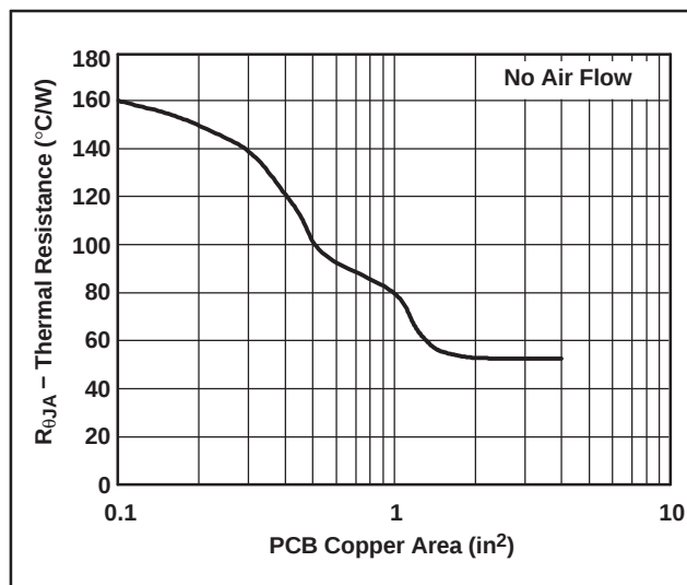
Figure 30. SOT223 Thermal Resistance vs PCB Copper Area
