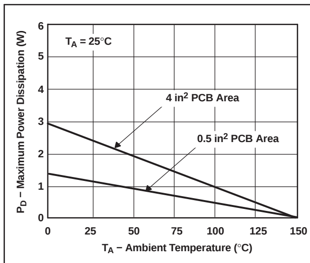
Figure 31. SOT223 Maximum Power Dissipation vs Ambient Temperature
