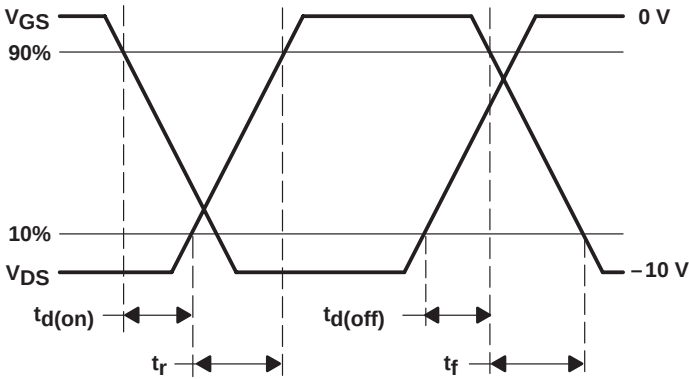
Figure 2. Switching-Time Waveforms
