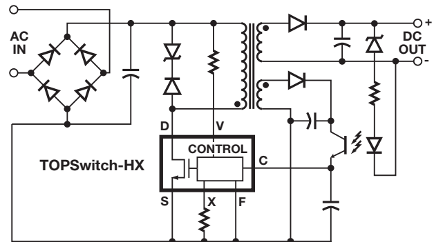
Figure 1. Typical Flyback Application.
