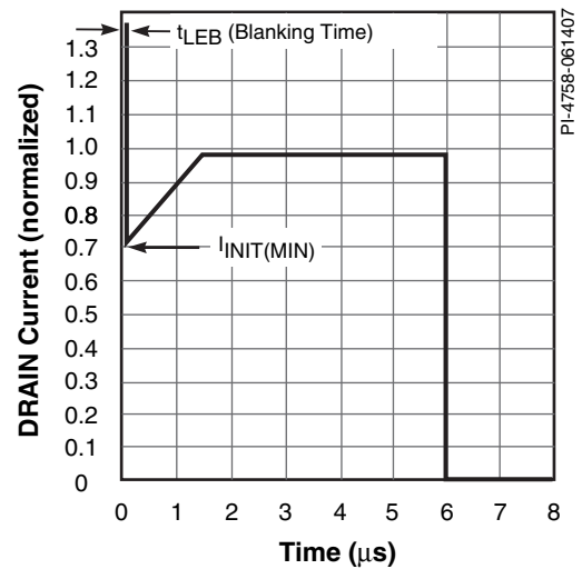
Figure 53. Drain Current Operating Envelope.
