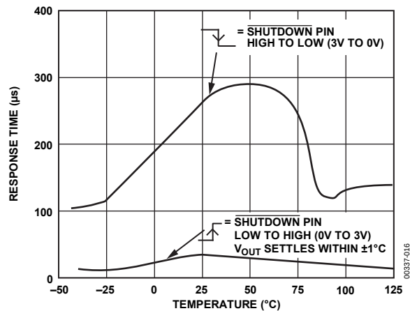
Figure 15. V_{OUT} Response Time for \overline{SHUTDOWN} Pin vs. Temperature
