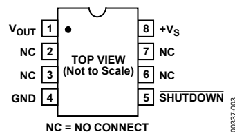
Figure 3. R-8 (SOIC_N)
