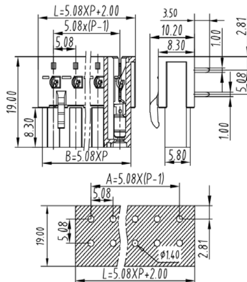
PCB Layout
