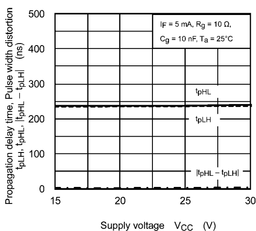
Fig. 12.2.15 t_{pHL} , t_{pLH} , |t_{pHL} - t_{pLH}| - V_{CC}
