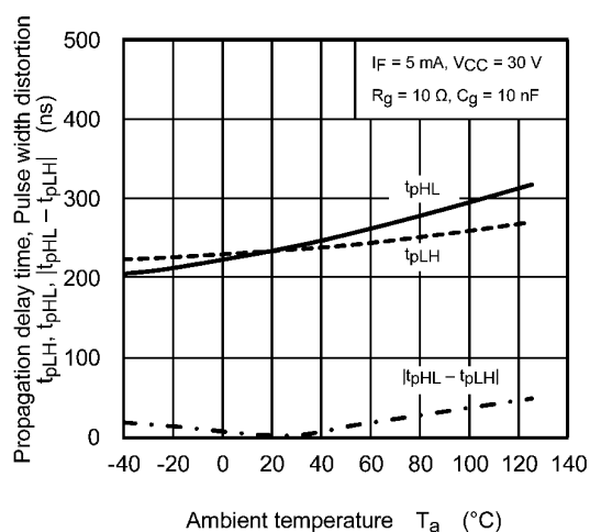
Fig. 12.2.13 t_{pHL} , t_{pLH} , |t_{pHL} - t_{pLH}| - T_a
