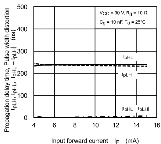
Fig. 12.2.14 t_{pHL} , t_{pLH} , |t_{pHL} - t_{pLH}| - I_F
