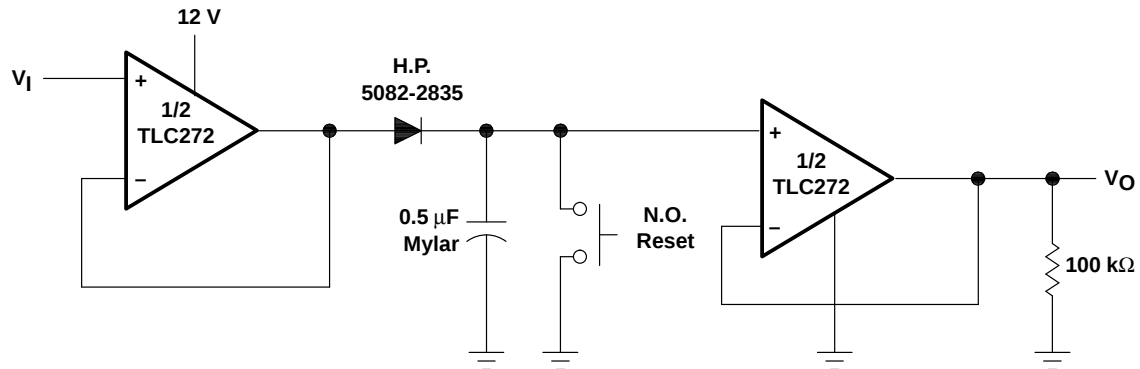
Figure 45. Positive-Peak Detector
