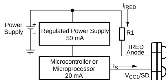
TFDU4100 (Note: Typical Values Listed) Receive Mode
