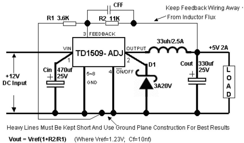
Figure 12. Typical Application of TD1509 For ADJ
