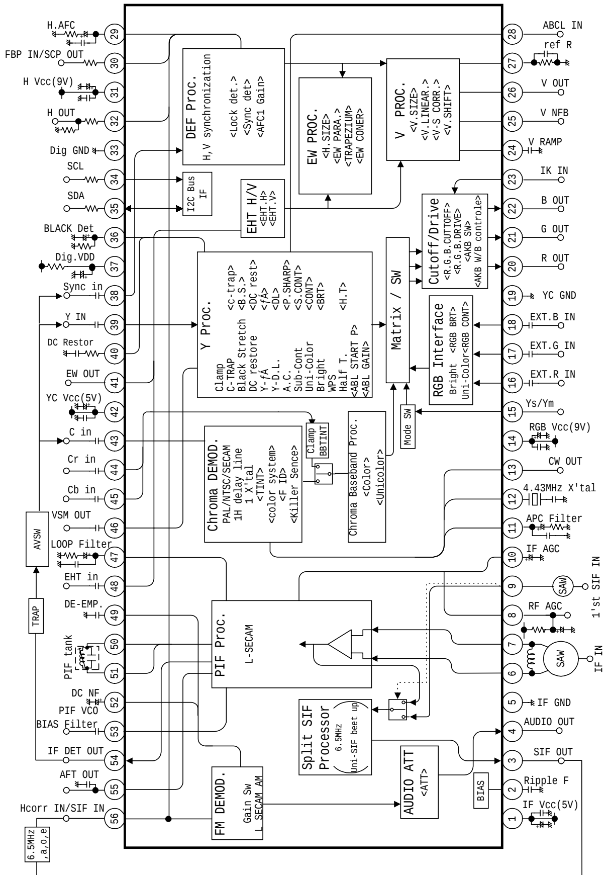
TB1251N BLOCK DIAGRAM
