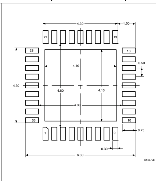
Figure 41. Recommended footprint (dimensions in mm) (1)(2)(3)
