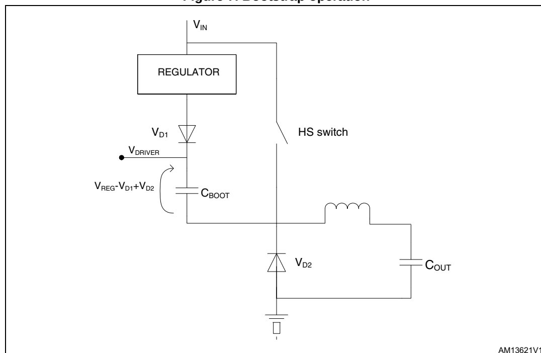
Figure 7. Bootstrap operation
