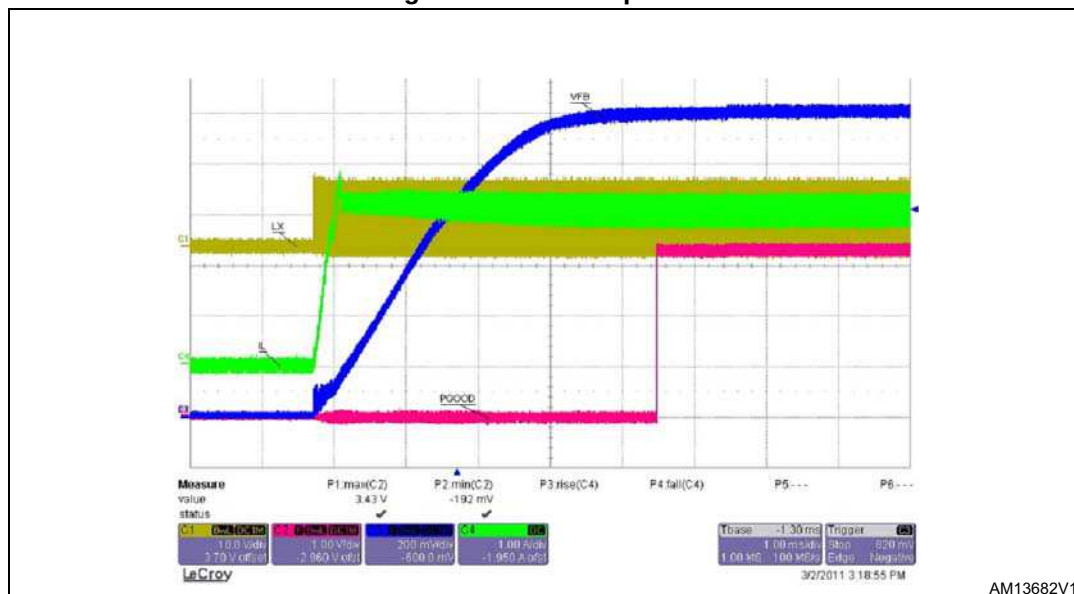
Figure 5. Soft-start phases
