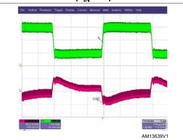
Figure 45. 1 A to 3 A falling edge load transient ( V_{IN} 24 V)
