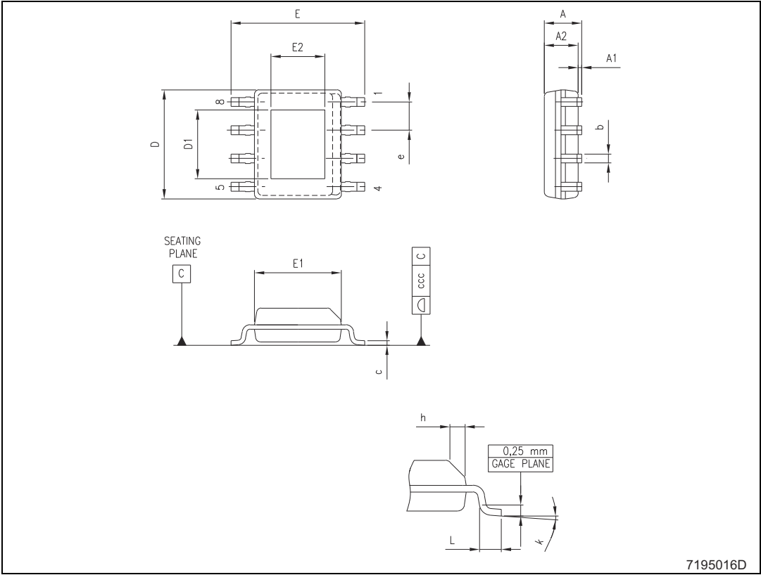
Figure 51. Package dimensions
