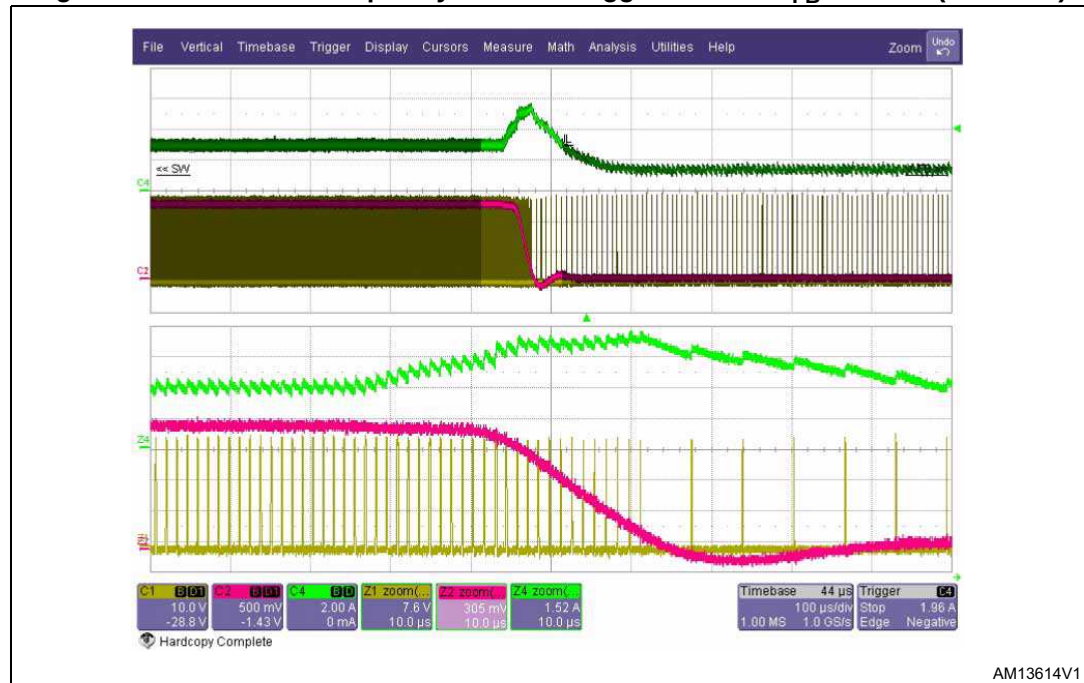
Figure 18. Current and frequency foldback triggered when V_{FB} < 300 mV (red trace)
