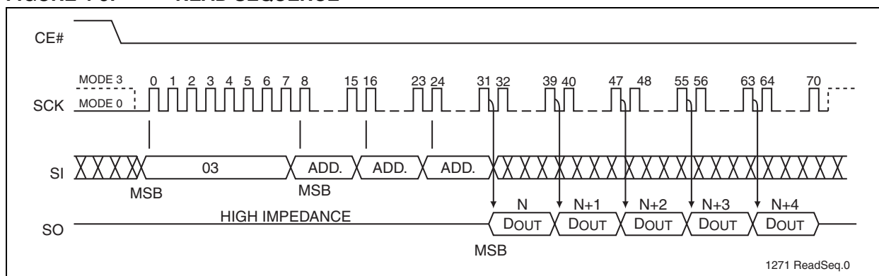
FIGURE 4-3: READ SEQUENCE
