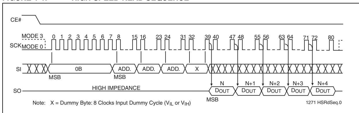
FIGURE 4-4: HIGH-SPEED-READ SEQUENCE
