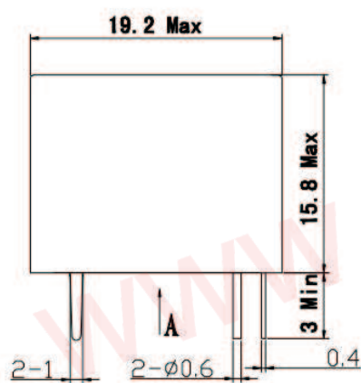
Physical installation diagram
