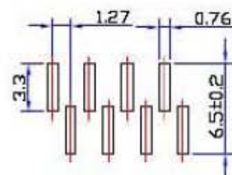
P.C Board Layout Type B
