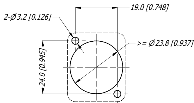
PANEL CUTOUT (1:1)
