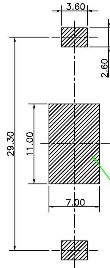
PCB LAYOUT
