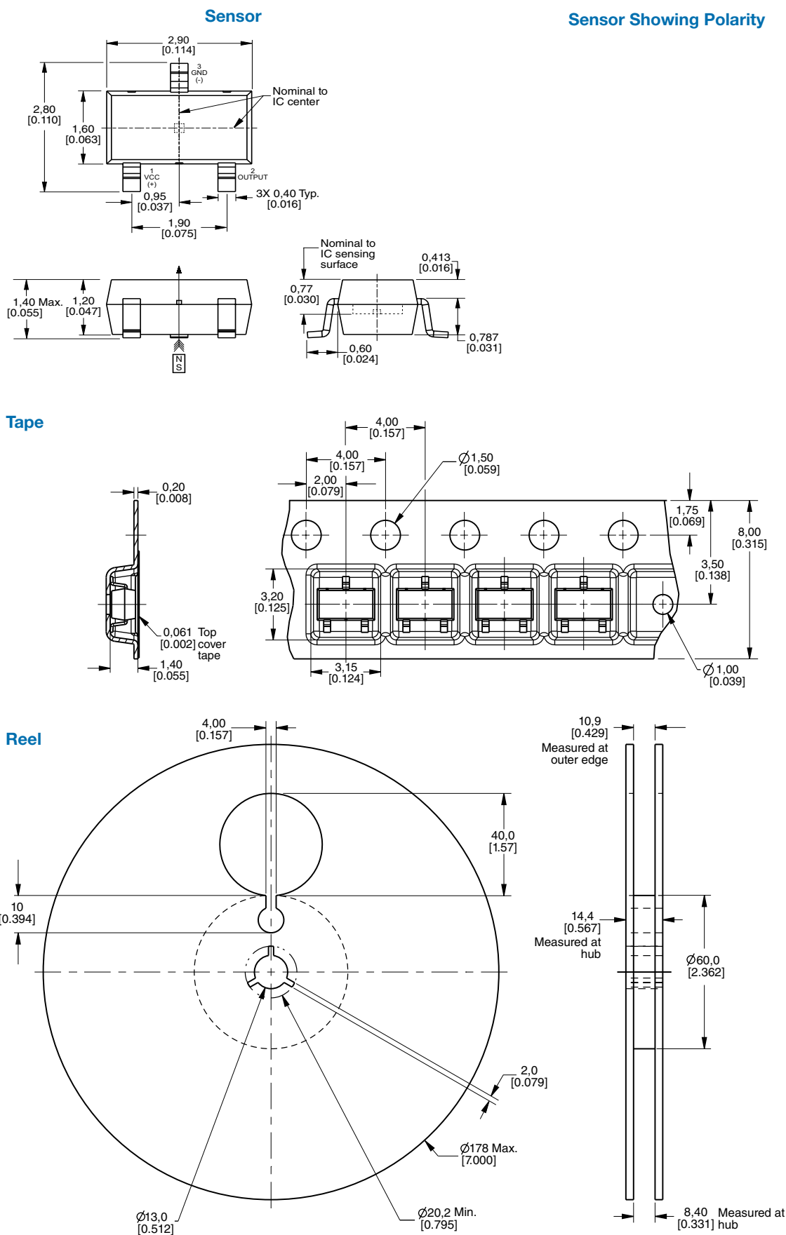
Figure 5. Mounting and Tape/Reel Dimensions (For reference only. mm/[in.] )
