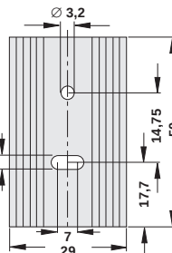
SK 09 50 TO 220
