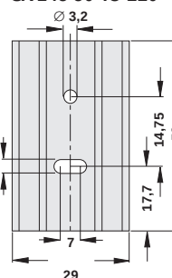
SK 145 50 TO 220
