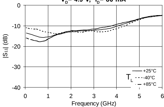
|S_{11}| vs. Frequency V_D = 4.9 \text{ V} , I_D = 80 \text{ mA}
