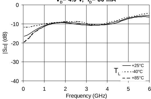
|S_{22}| vs. Frequency V_D = 4.9 \text{ V} , I_D = 80 \text{ mA}
