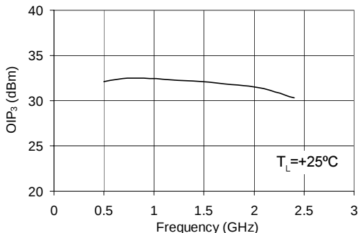
OIP 3 vs. Frequency V_D = 4.9\text{ V} , I_D = 80\text{ mA}
