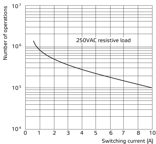
Electrical endurance
