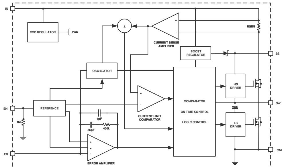
RY8310 Block Diagram
