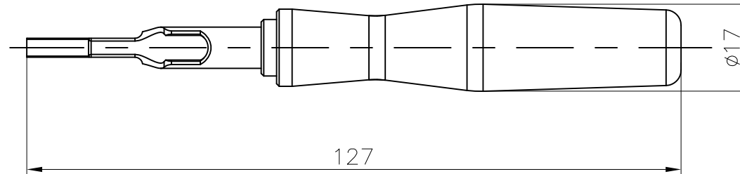
Contact removal tool Application:16A Crimp contacts
