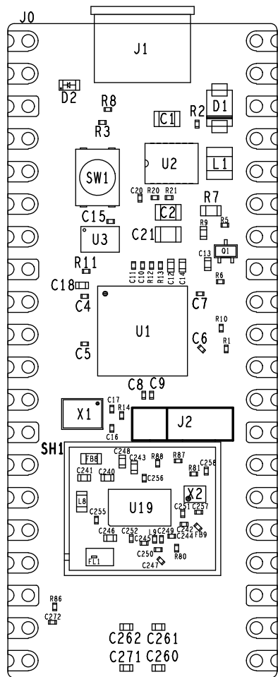
Figure 12. The Pico W Rev3 board component locations.
