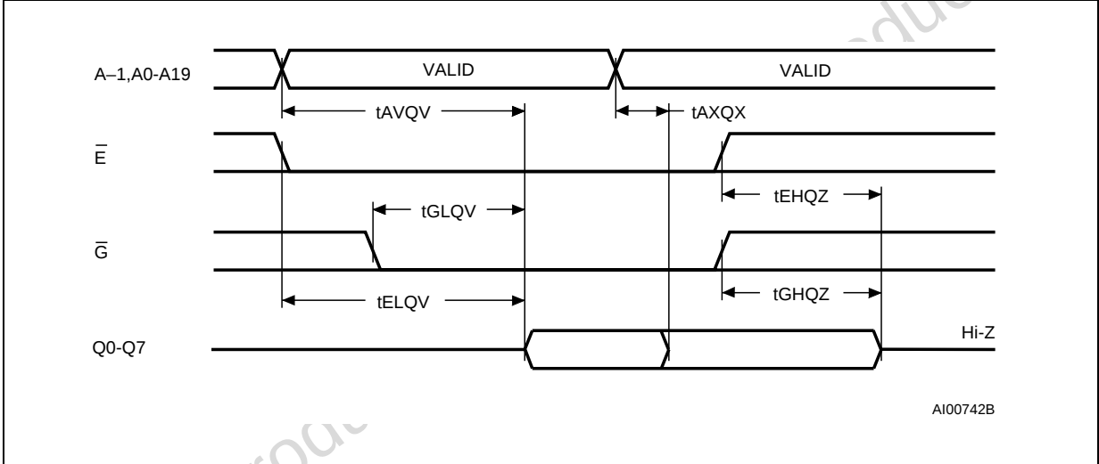
Figure 9. Byte-Wide Read Mode AC Waveforms
