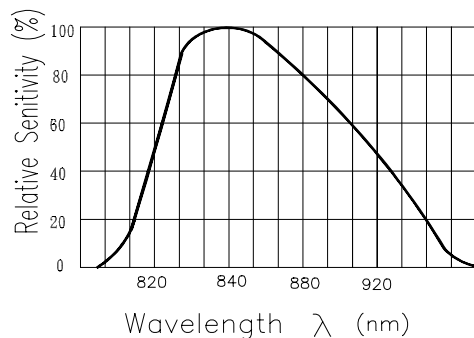
Fig.5 Spectral Sensitivity
