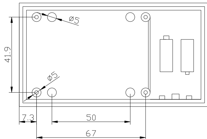
Tapa Interior
