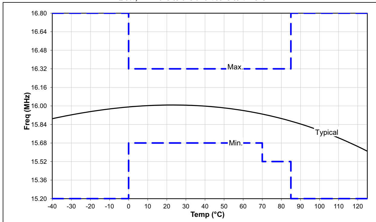
FIGURE 28-100: PIC18(L)F2X/4XK22 HF-INTOSC FREQUENCY vs. TEMPERATURE at 16 MHz MIN / MAX: \pm 2\% , T = 0^{\circ}\text{C} to +70^{\circ}\text{C} +2\% / -3\% , T = +70^{\circ}\text{C} to +85^{\circ}\text{C} \pm 5\% , T = -40^{\circ}\text{C} to 0^{\circ}\text{C} and +85^{\circ}\text{C} to +125^{\circ}\text{C}
