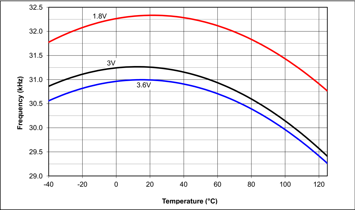
FIGURE 28-103: PIC18LF2X/4XK22 TYPICAL LF-INTOSC FREQUENCY vs. TEMPERATURE Min/Max = 31.25 kHz \pm 15%, T = -40 ^{\circ} C to +85 ^{\circ} C
