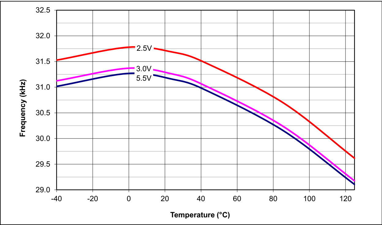
FIGURE 28-104: PIC18F2X/4XK22 TYPICAL LF-INTOSC FREQUENCY vs. TEMPERATURE Min/Max = 31.25 kHz \pm 15%, T = -40 ^{\circ} C to +85 ^{\circ} C
