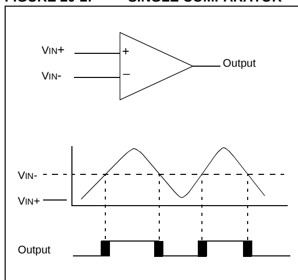
FIGURE 20-2: SINGLE COMPARATOR
