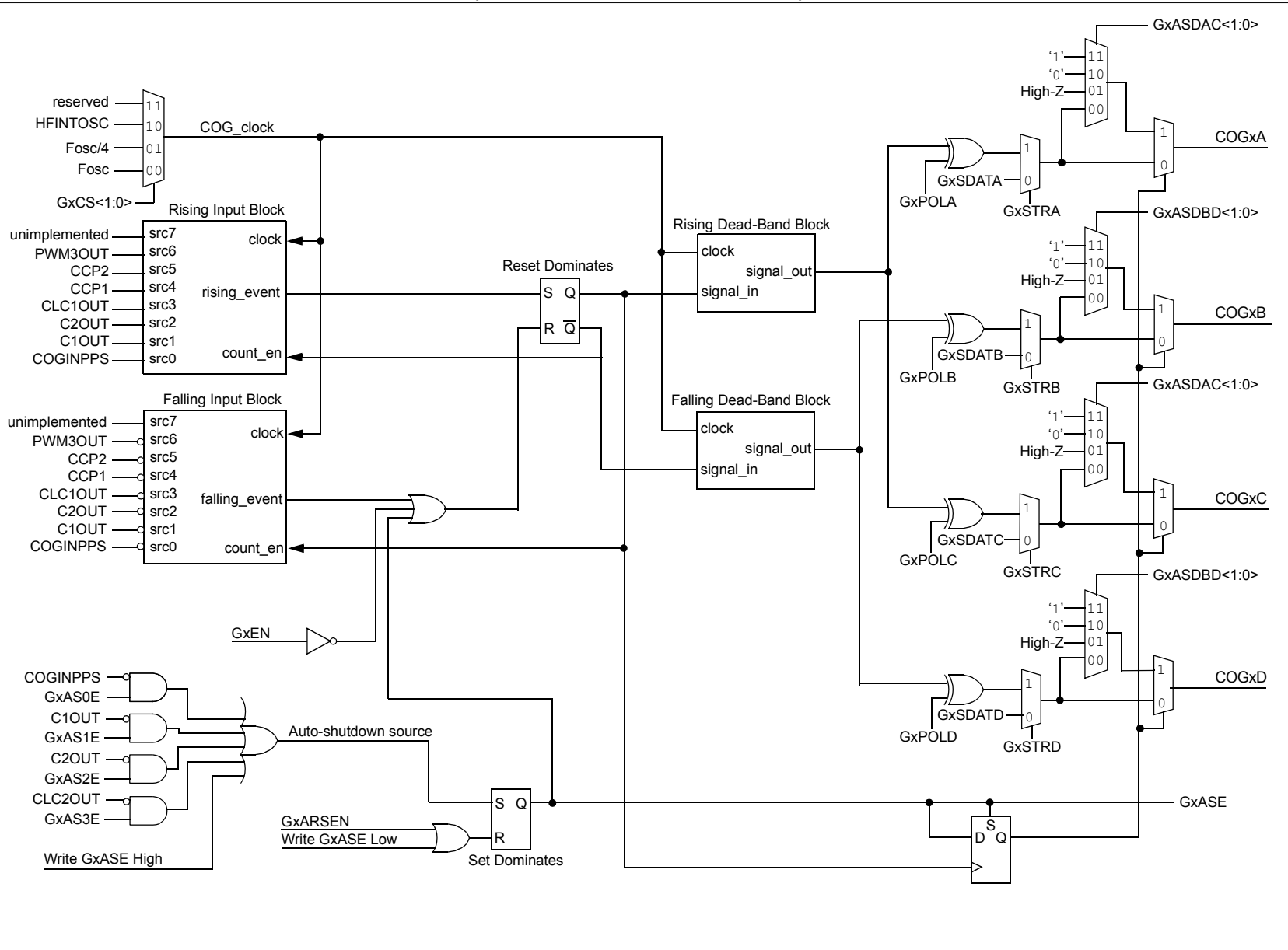
FIGURE 18-5: SIMPLIFIED COG BLOCK DIAGRAM (HALF-BRIDGE MODE, GXMD = 4)
