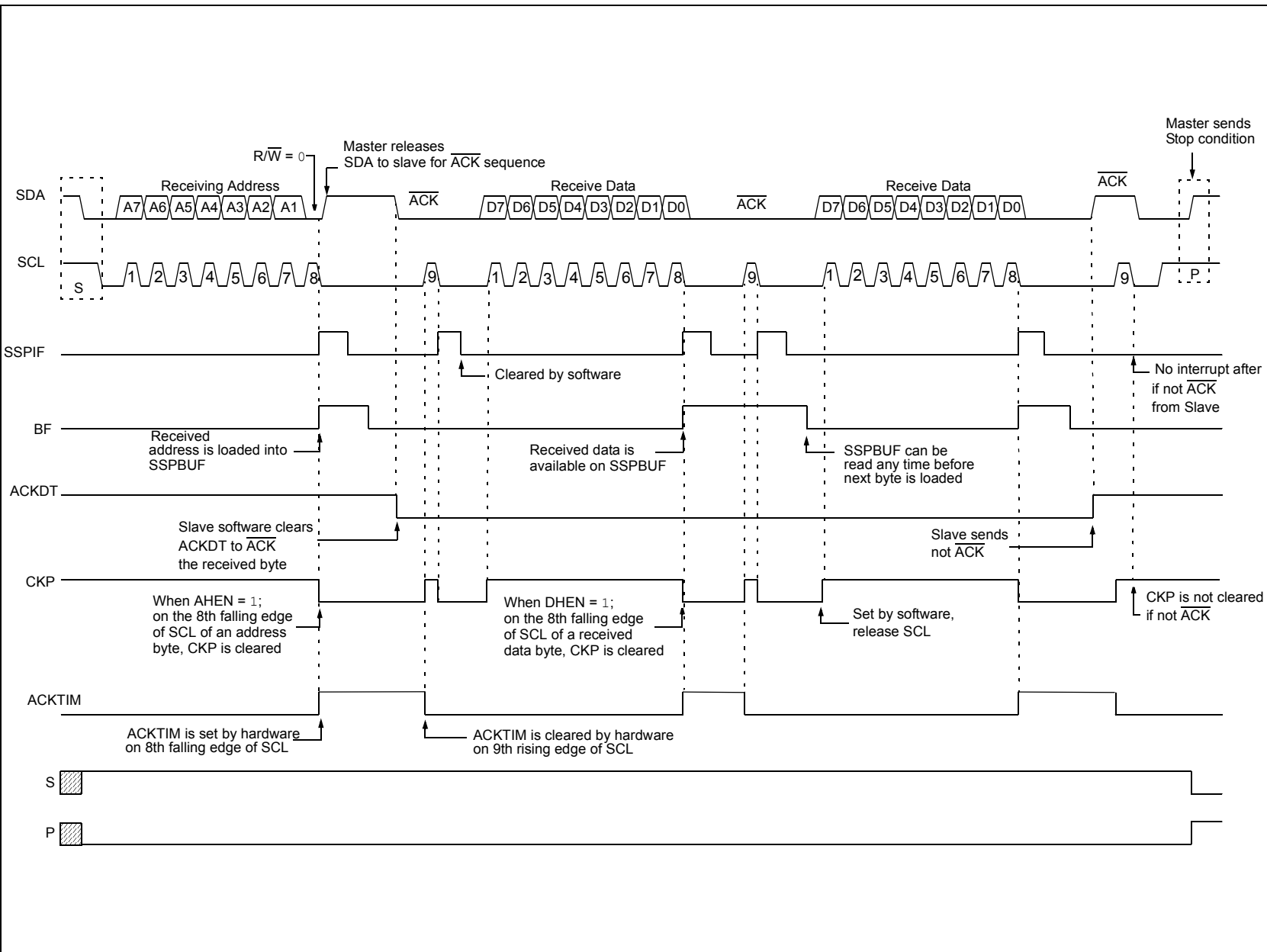
FIGURE 28-17: I 2 C SLAVE, 7-BIT ADDRESS, RECEPTION (SEN = 1, AHEN = 1, DHEN = 1)
