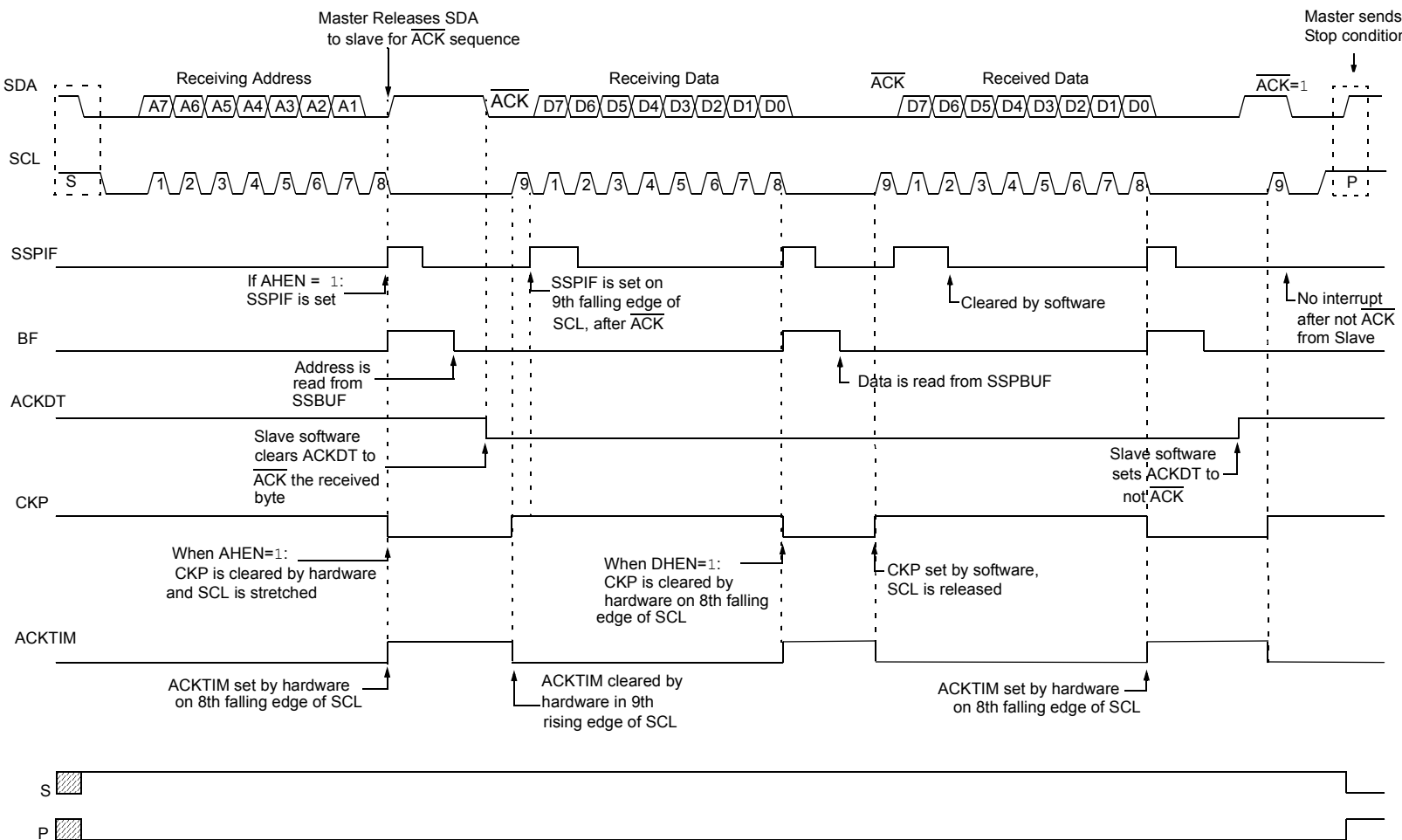
FIGURE 28-16: I 2 C SLAVE, 7-BIT ADDRESS, RECEPTION (SEN = 0, AHEN = 1, DHEN = 1)
