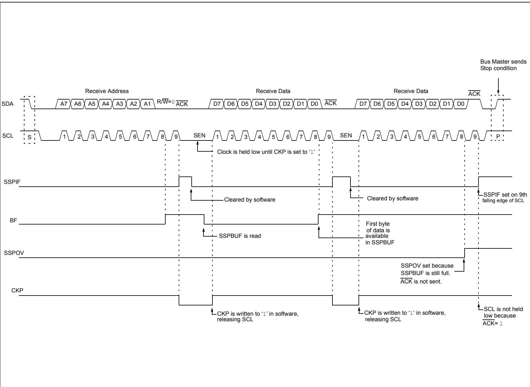
FIGURE 28-15: I 2 C SLAVE, 7-BIT ADDRESS, RECEPTION (SEN = 1, AHEN = 0, DHEN = 0)
