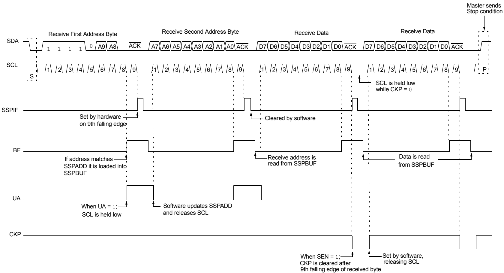
FIGURE 28-20: I 2 C SLAVE, 10-BIT ADDRESS, RECEPTION (SEN = 1, AHEN = 0, DHEN = 0)
