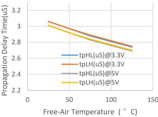
Figure11. Propagation Delay Time vs. Free-Air Temperature
