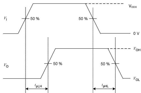
Figure16. Propagation delay time waveform measurement
