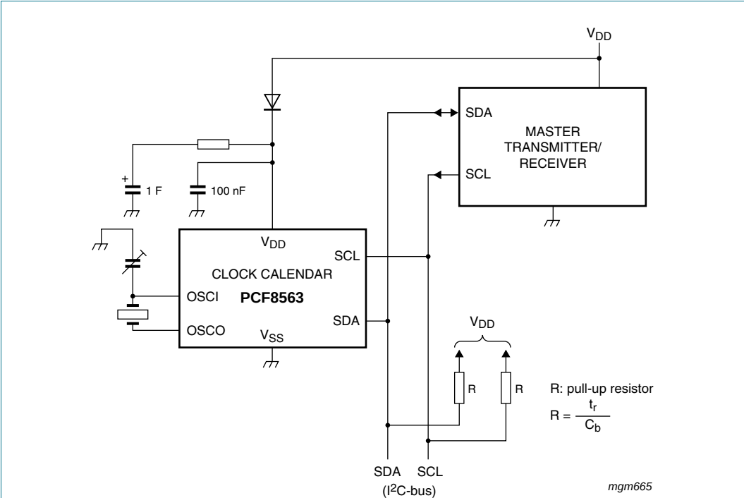
Fig 29. Application diagram
