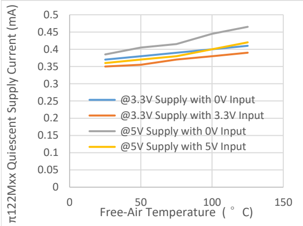
Figure 12. \pi 121\text{Mxx}/\pi 122\text{Mxx} Quiescent Supply Current vs. Free-Air Temperature
