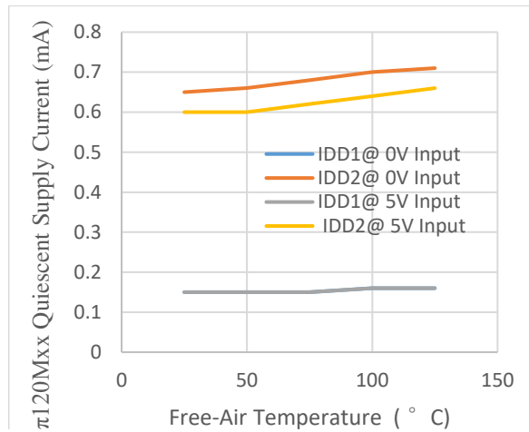
Figure 14. \pi 120\text{Mxx} Quiescent Supply Current with 5V Supply vs. Free-Air Temperature
