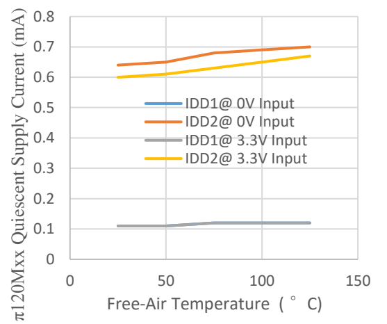
Figure 13. \pi 120\text{Mxx} Quiescent Supply Current with 3.3V Supply vs. Free-Air Temperature
