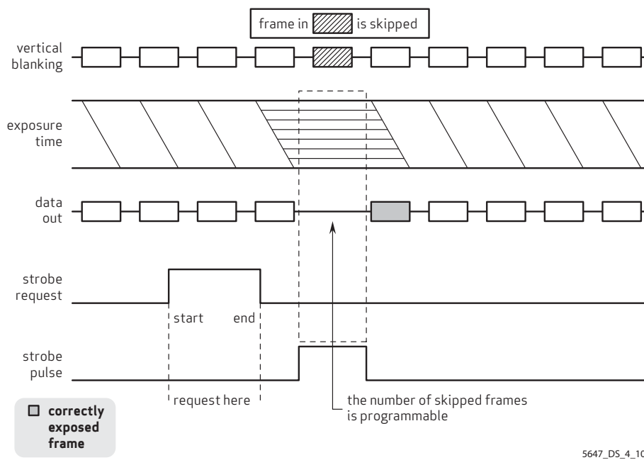
figure 4-10 LED 1 & 2 mode - one pulse output
