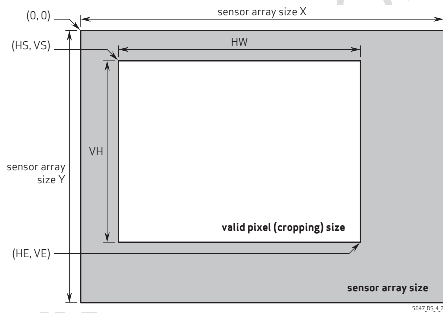
figure 4-2 image windowing
