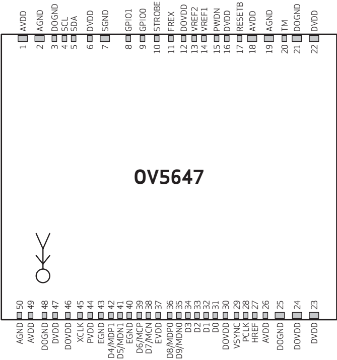
figure 1-1 pad diagram
