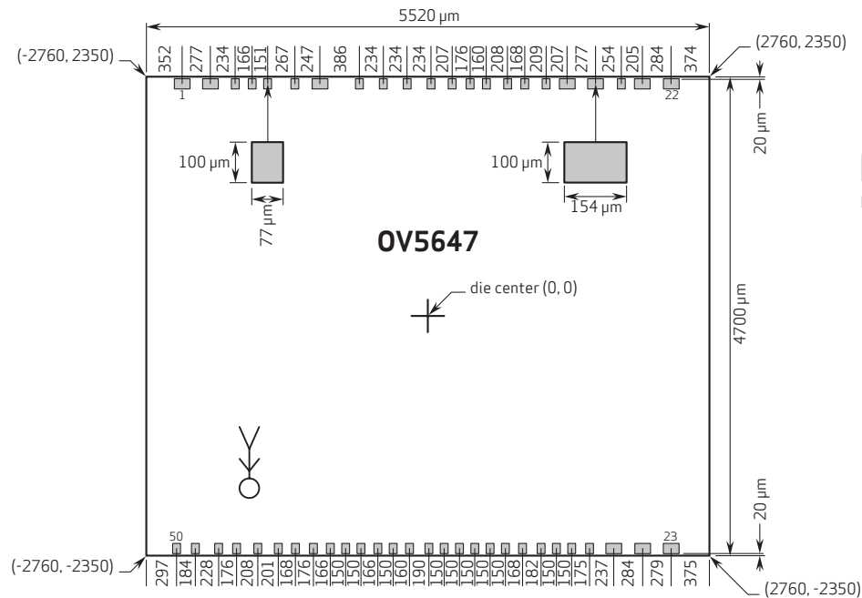
figure 9-1 die specifications
